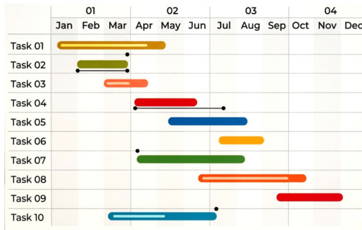
Fig. 2.1.2 Gantt Chart
