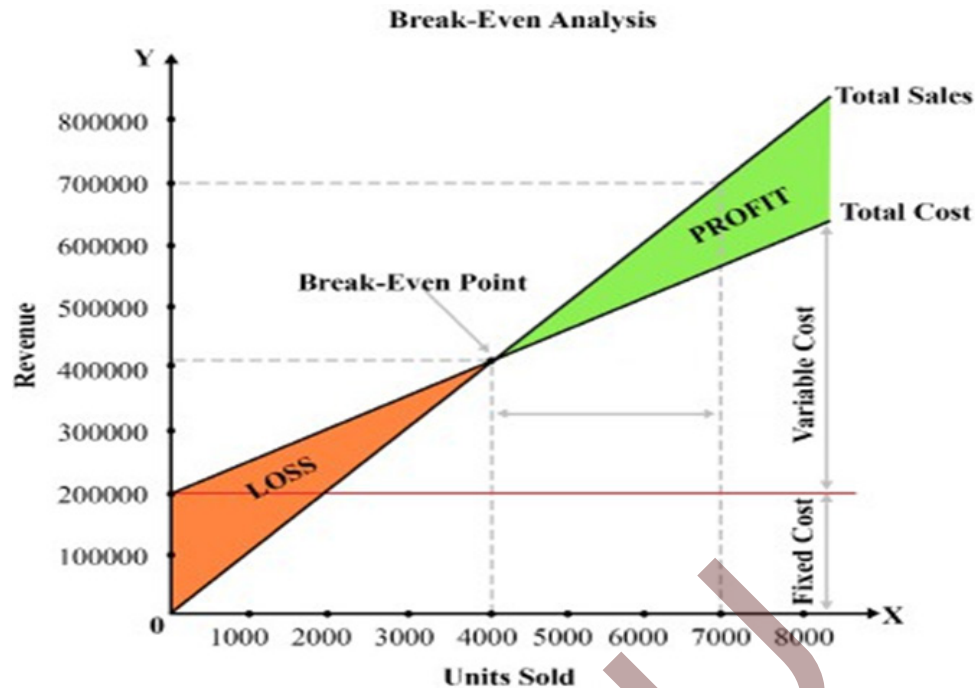
Figure 2.2.10 Break-Even Analysis
